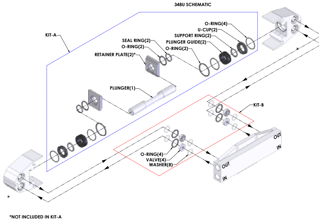
Figure 12 – repair Parts illustration for Plunger Pump
